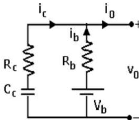
Fig.1 Equivalent Circuit
